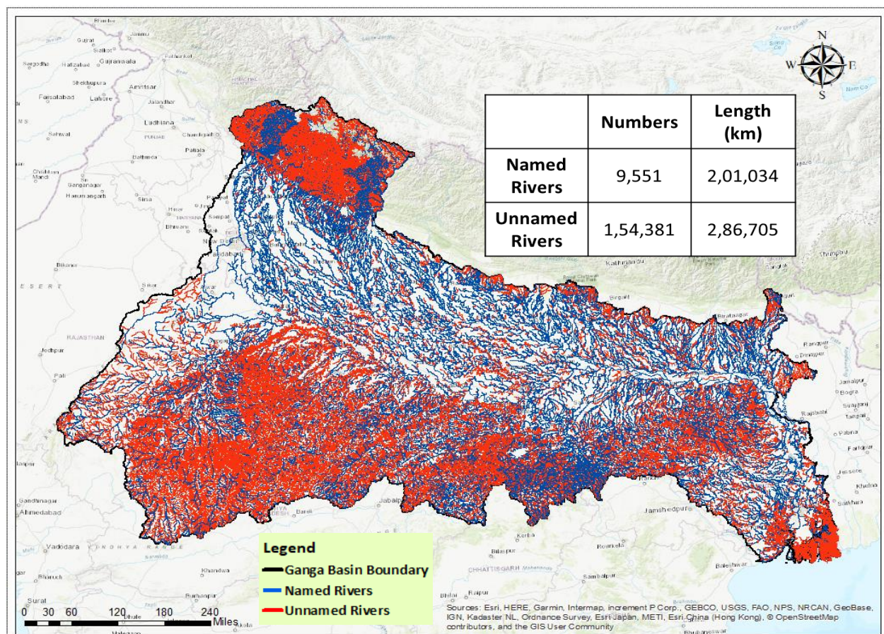
Figure 5: Spatial Distribution of Rivers in the Ganga Basin
